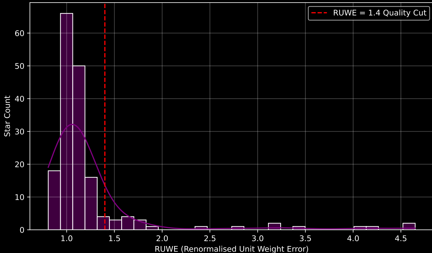
GAPOGEE DR17 Field [271-34-O_TESS] RUWE Distribution (n= 174)
