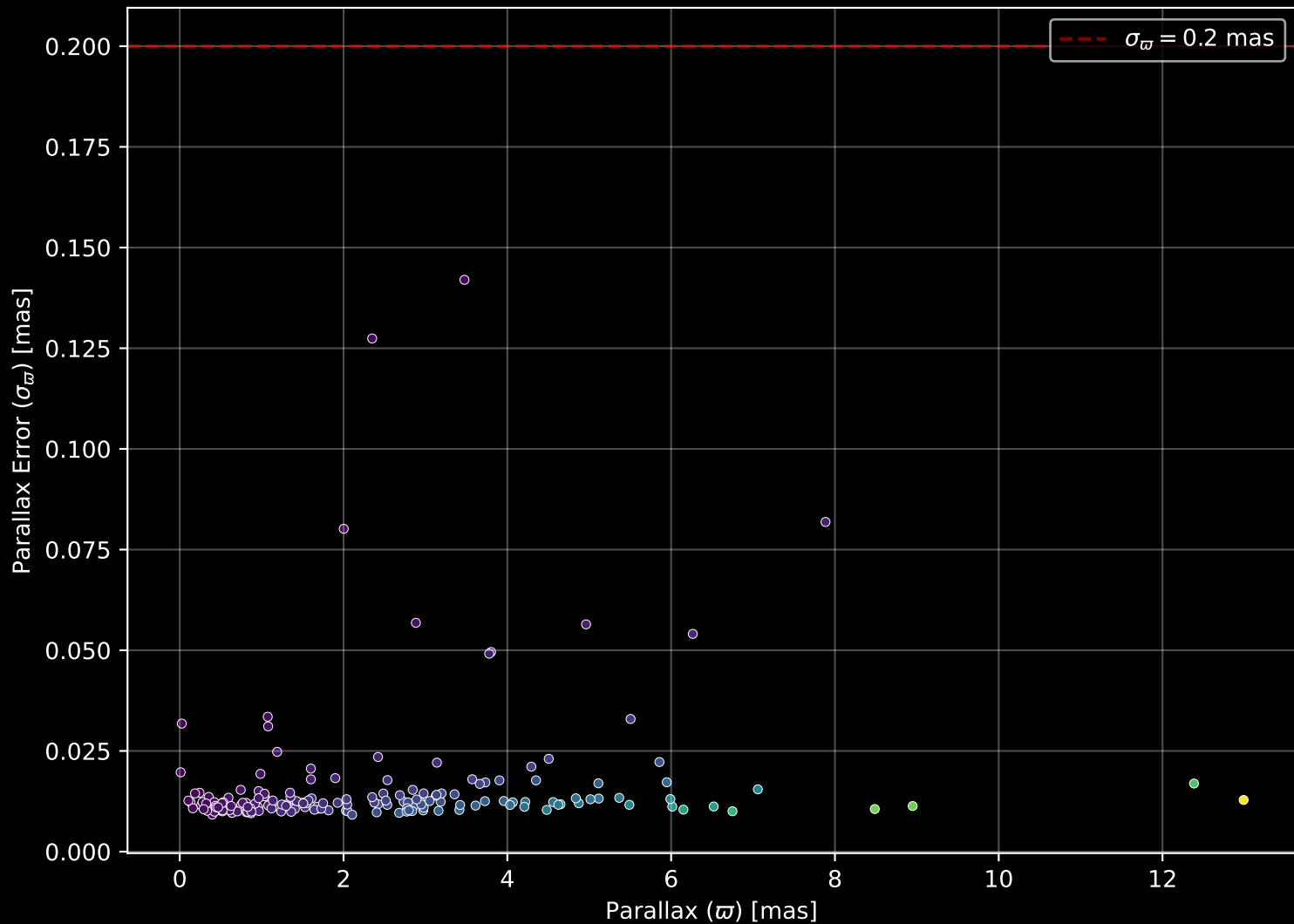
APOGEE DR17 Field: [271-34-O_TESS] Parallax Quality (n= 177)
