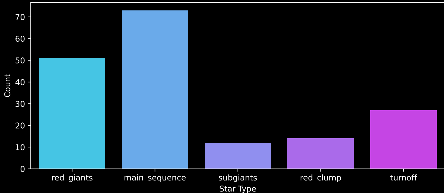
APOGEE DR17 Field: [271-34-O_TESS] Count plot of Star Type
