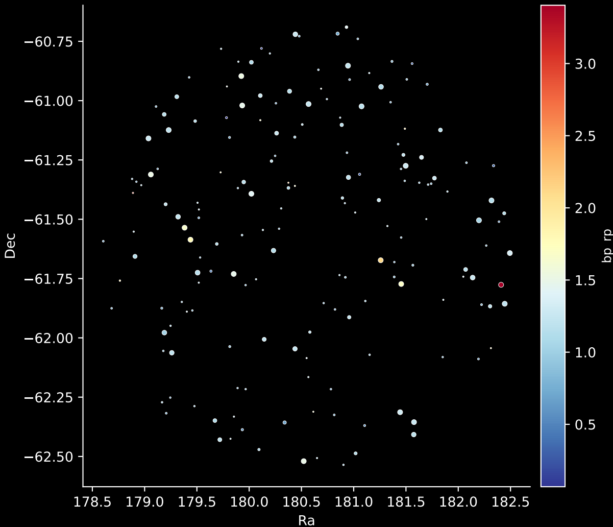
APOGEE DR17 Field: [271-34-O_TESS] Stars: 177
