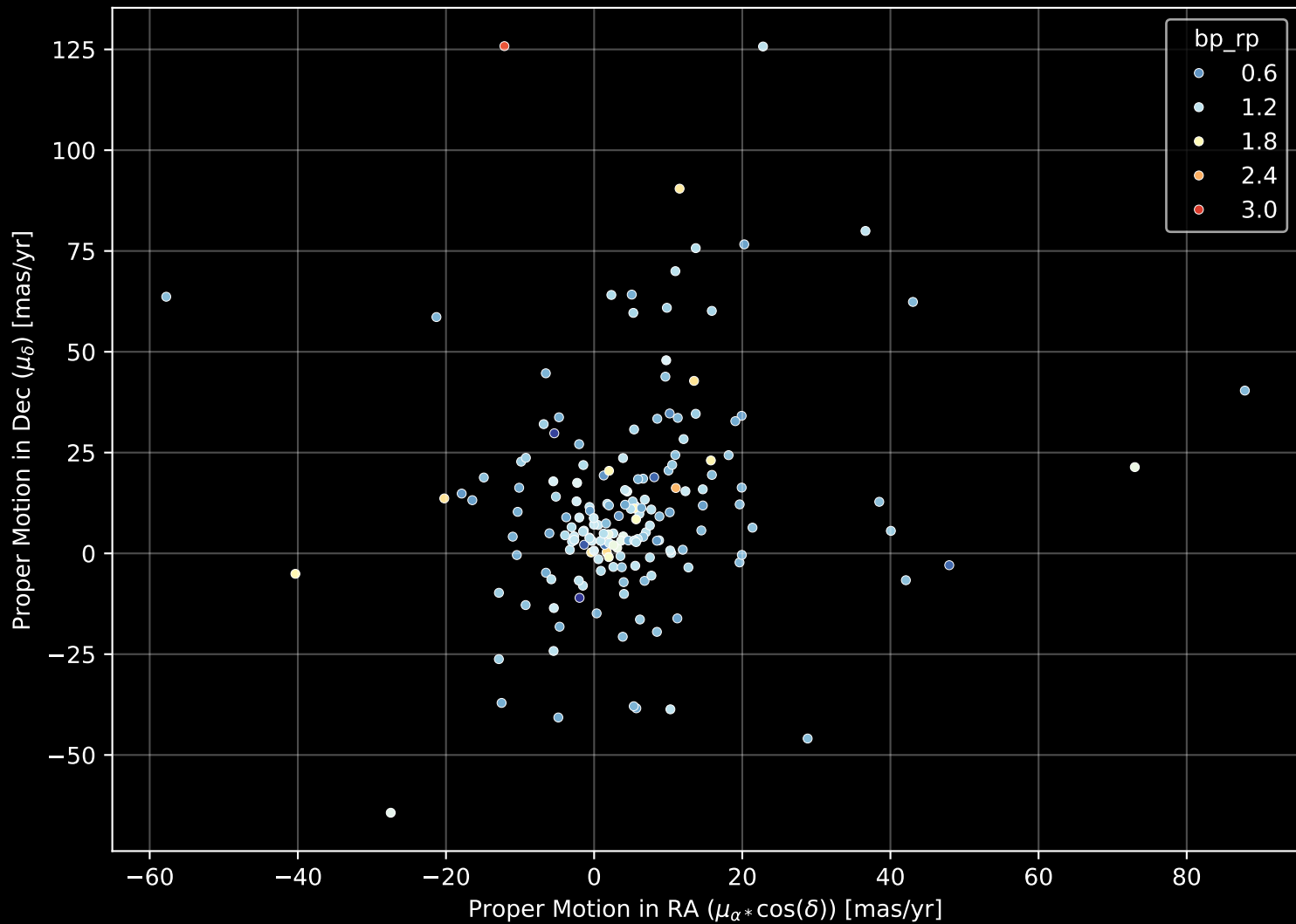
APOGEE DR17 Field: [271-34-O_TESS] Proper Motion Diagram (n= 177)
